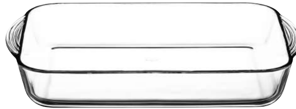
RECTANGULAR TRAY DİKDÖRTGEN TEPSİ 59124 ~3850 cc. 128 1/4 US oz. - 135 2/4 UK oz. 60 mm. 2 1/4" - - 400 x 250 mm. 15 3/4 x 9 3/4" 1043141 • gb1-4ob/hk1-4dk
